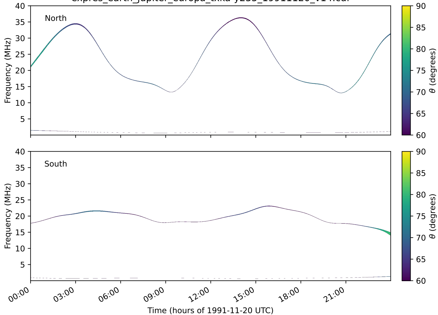
expres_earth_jupiter_europa_txka-y235_19911120_v14.cdf
