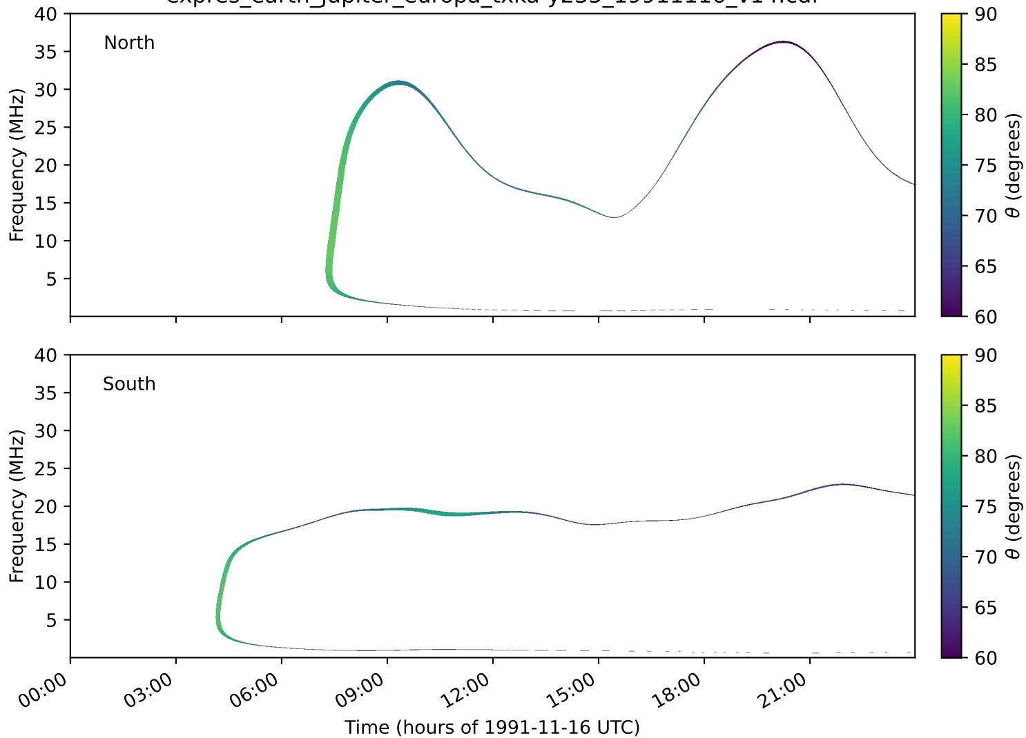
expres_earth_jupiter_europa_txka-y235_19911116_v14.cdf
