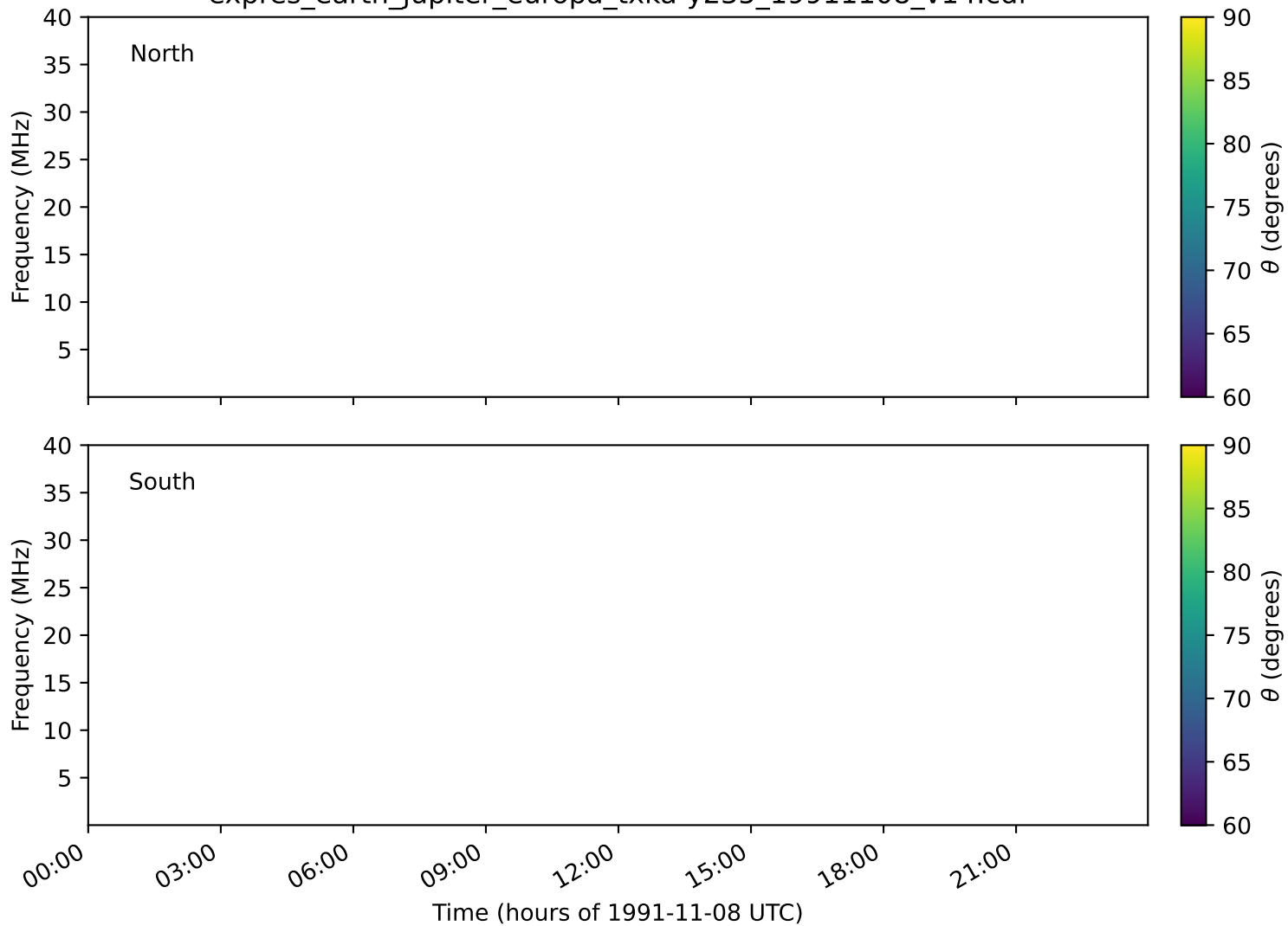
expres_earth_jupiter_europa_txka-y235_19911108_v14.cdf
