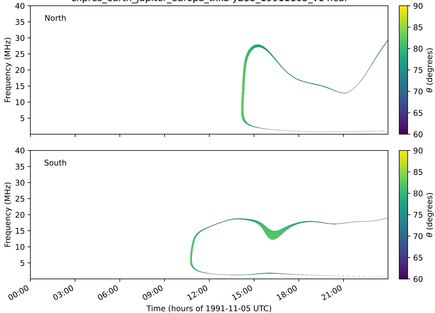
expres_earth_jupiter_europa_txka-y235_19911105_v14.cdf
