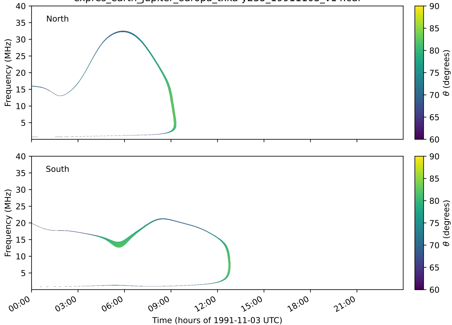
expres_earth_jupiter_europa_txka-y235_19911103_v14.cdf
