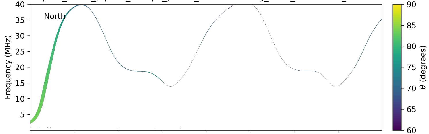
expres_earth_jupiter_europa_jrm33_lossc-wid1deg_3kev_19911127_v11.cdf
