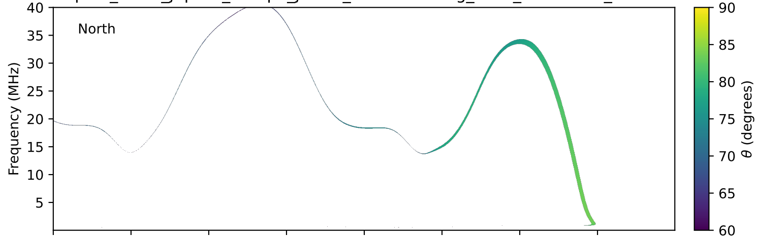
expres_earth_jupiter_europa_jrm33_lossc-wid1deg_3kev_19911124_v11.cdf
