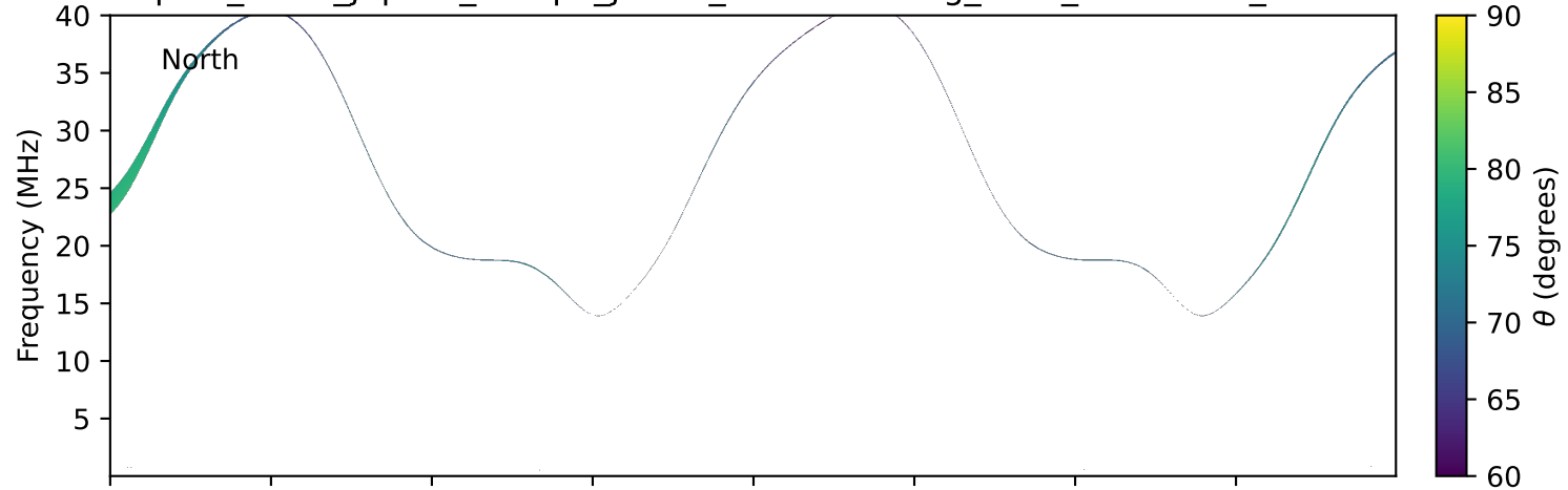
expres_earth_jupiter_europa_jrm33_lossc-wid1deg_3kev_19911120_v11.cdf
