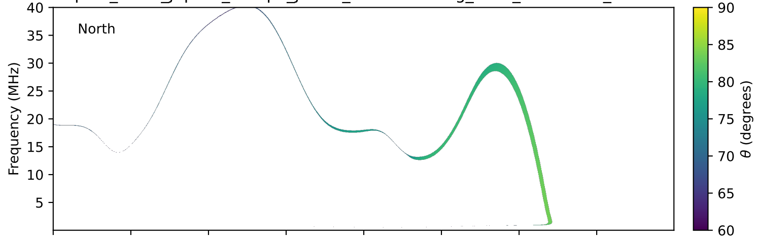
expres_earth_jupiter_europa_jrm33_lossc-wid1deg_3kev_19911117_v11.cdf
