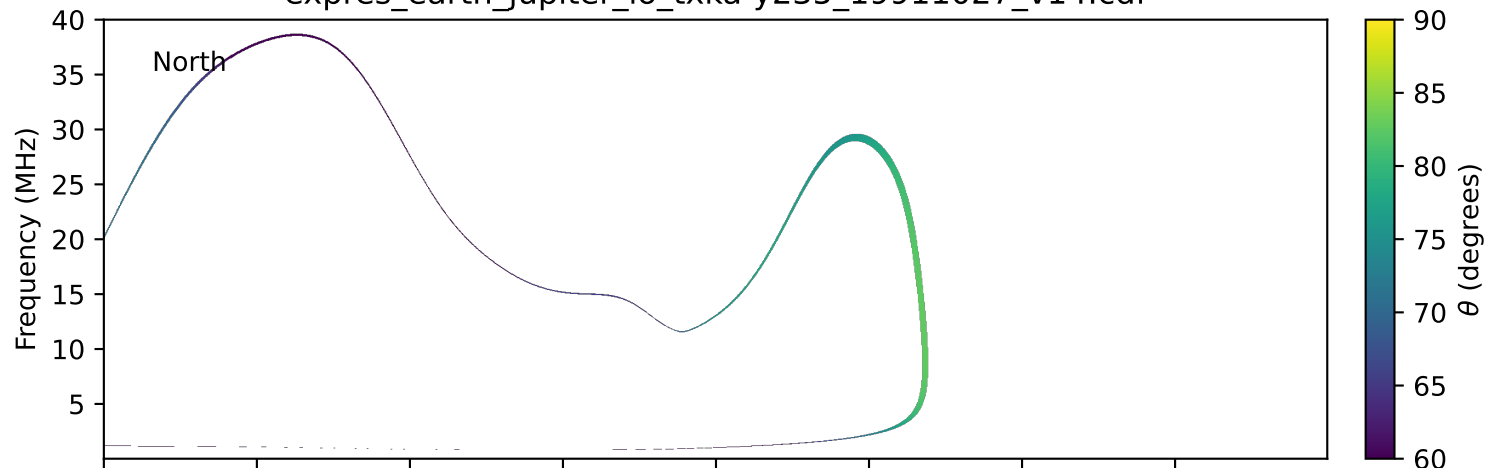
expres_earth_jupiter_io_txka-y235_19911027_v14.cdf
