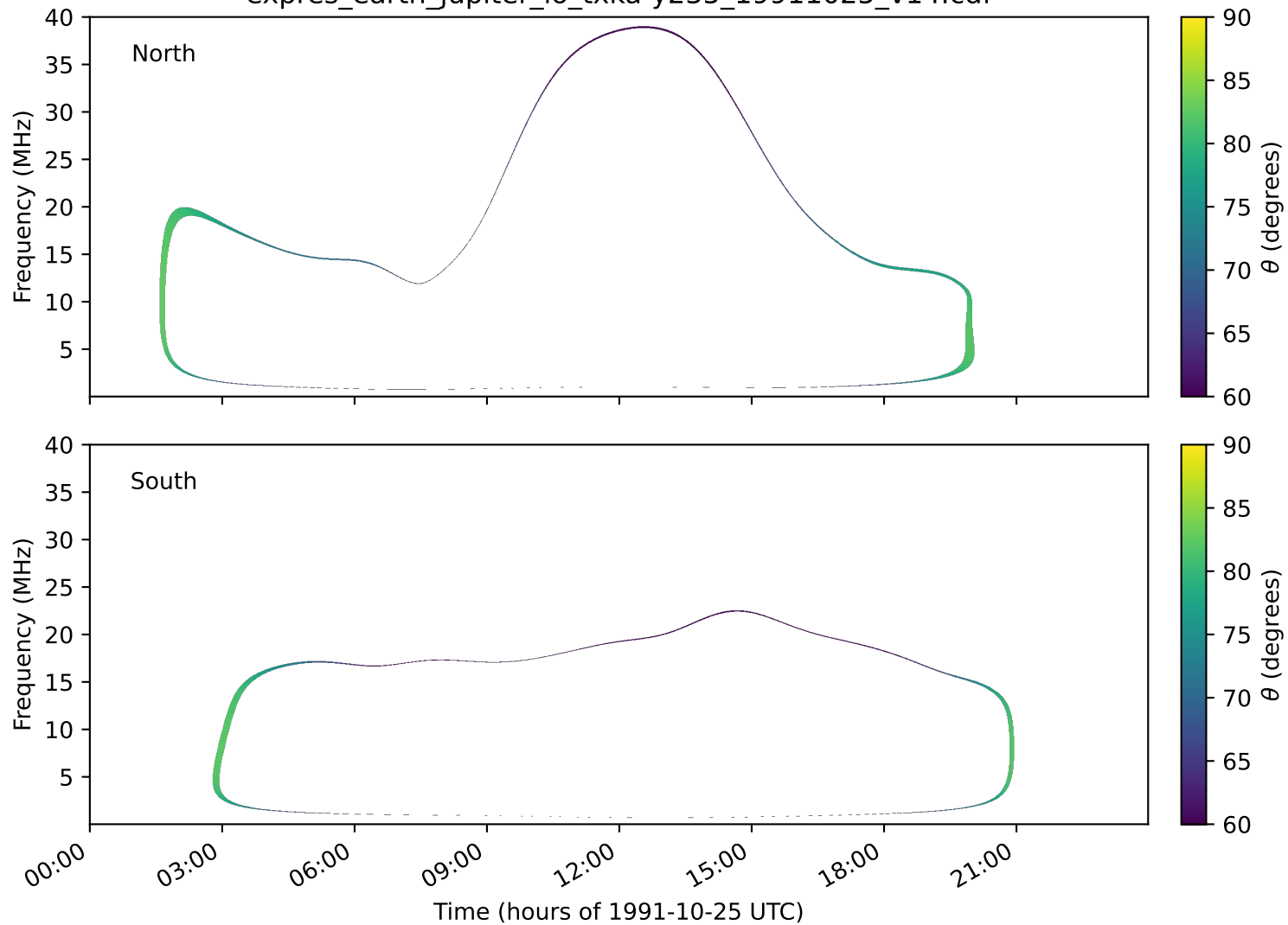
expres_earth_jupiter_io_txka-y235_19911025_v14.cdf
