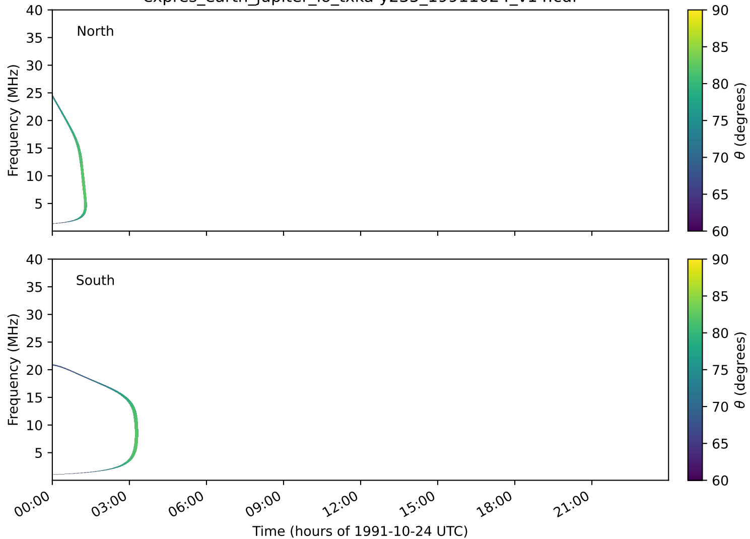
expres_earth_jupiter_io_txka-y235_19911024_v14.cdf
