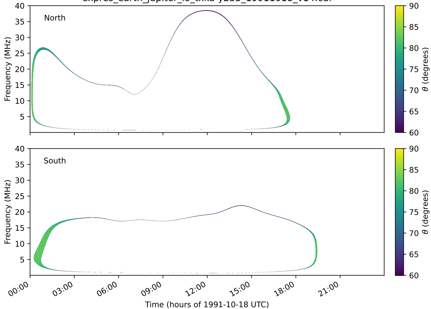
expres_earth_jupiter_io_txka-y235_19911018_v14.cdf
