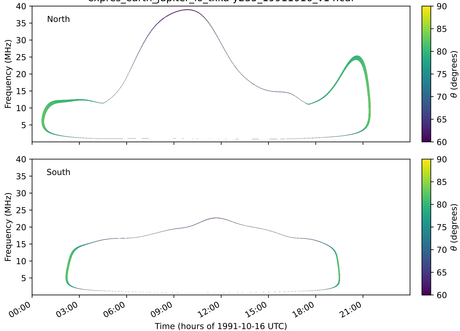
expres_earth_jupiter_io_txka-y235_19911016_v14.cdf
