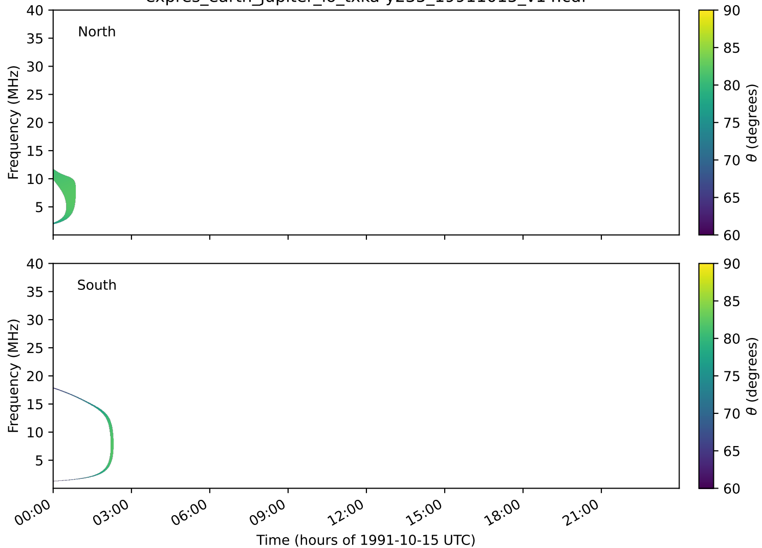
expres_earth_jupiter_io_txka-y235_19911015_v14.cdf
