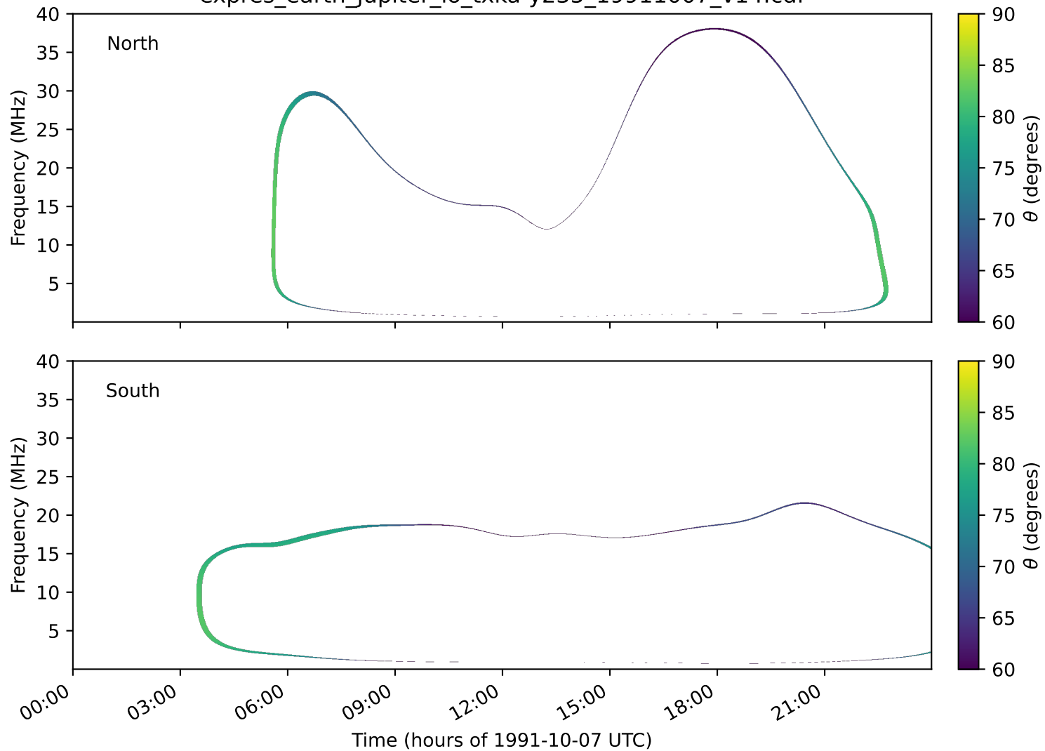
expres_earth_jupiter_io_txka-y235_19911007_v14.cdf
