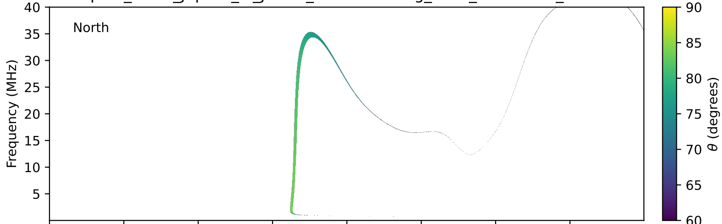
expres_earth_jupiter_io_jrm33_lossc-wid1deg_3kev_19911030_v11.cdf
