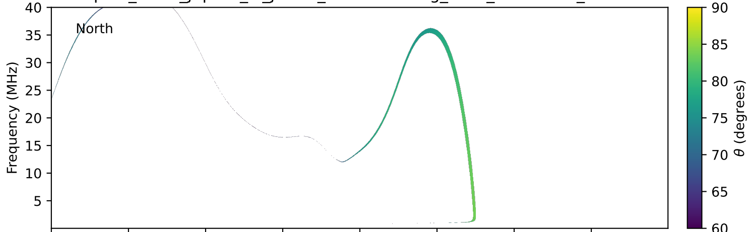
expres_earth_jupiter_io_jrm33_lossc-wid1deg_3kev_19911027_v11.cdf
