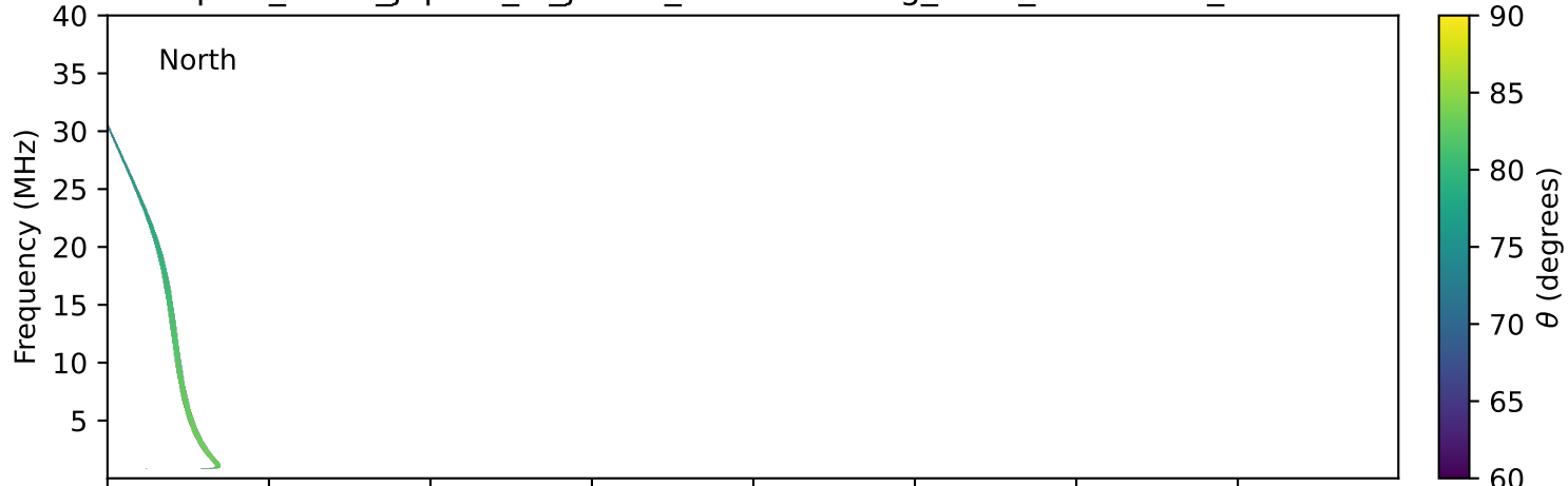
expres_earth_jupiter_io_jrm33_lossc-wid1deg_3kev_19911024_v11.cdf
