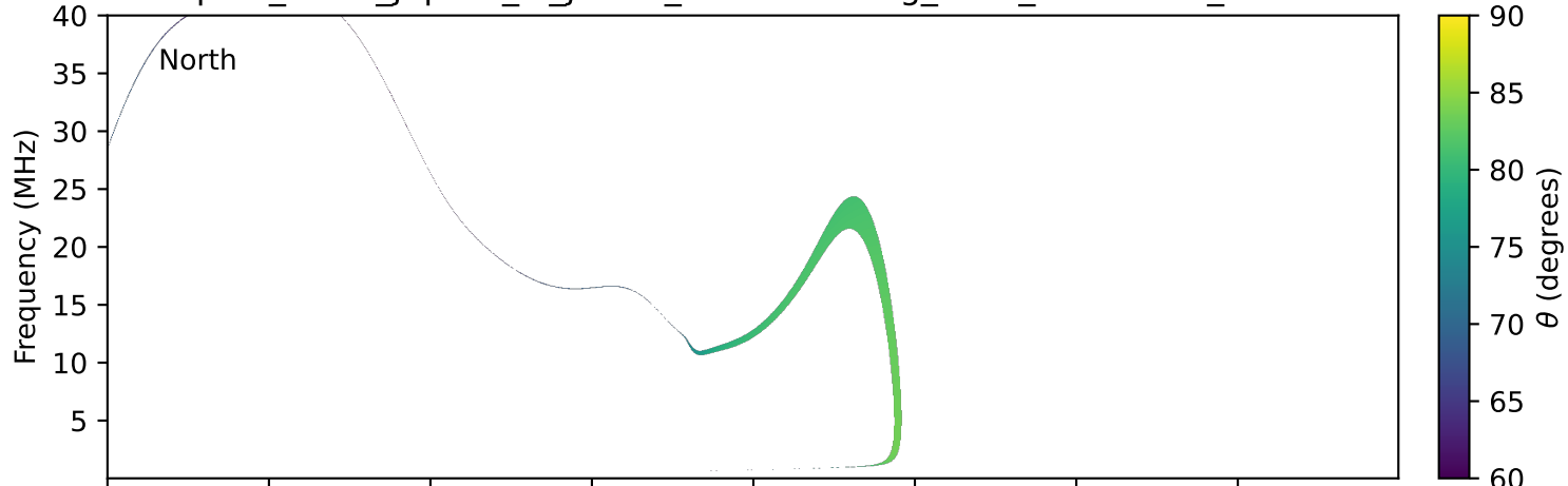
expres_earth_jupiter_io_jrm33_lossc-wid1deg_3kev_19911020_v11.cdf
