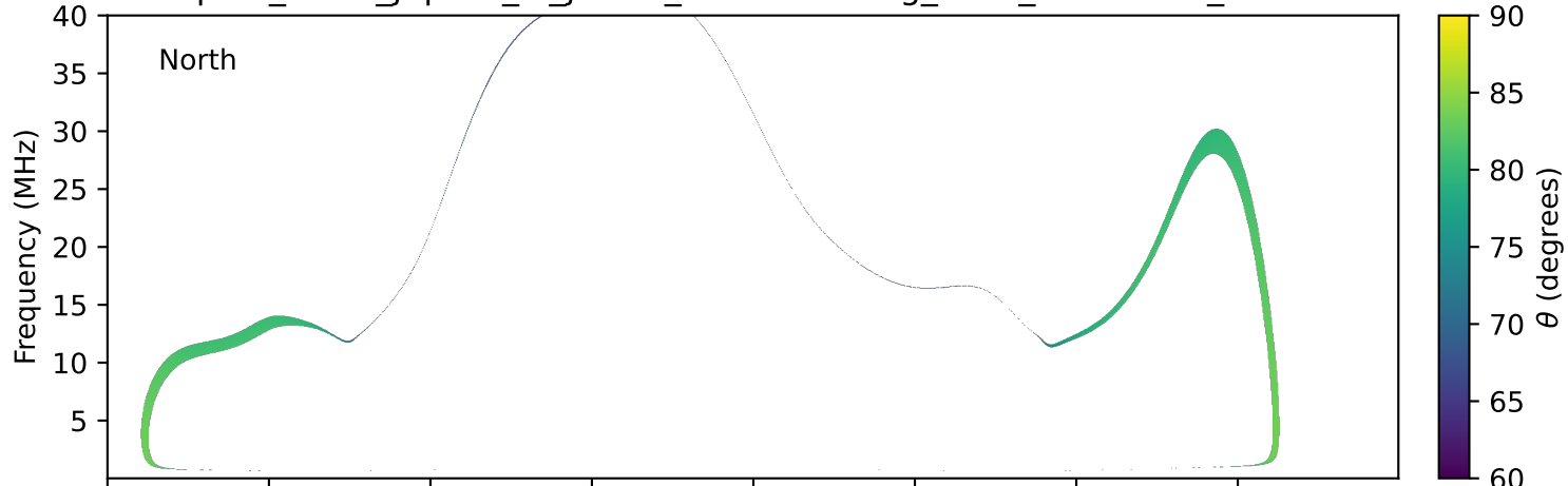
expres_earth_jupiter_io_jrm33_lossc-wid1deg_3kev_19911016_v11.cdf
