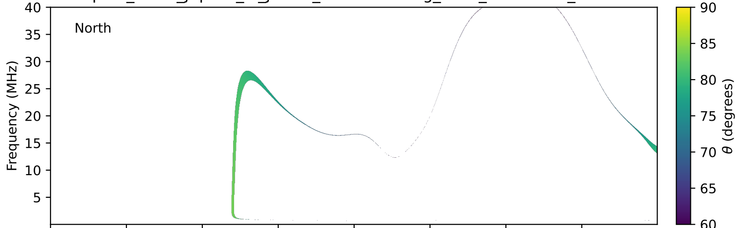
expres_earth_jupiter_io_jrm33_lossc-wid1deg_3kev_19911014_v11.cdf
