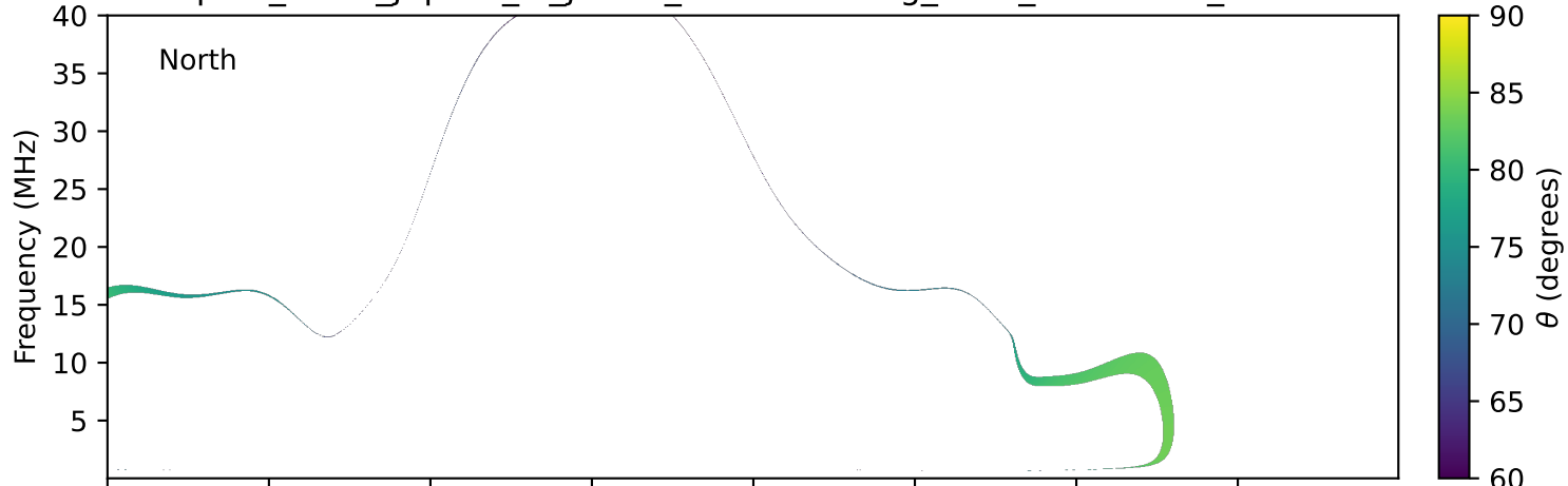
expres_earth_jupiter_io_jrm33_lossc-wid1deg_3kev_19911009_v11.cdf
