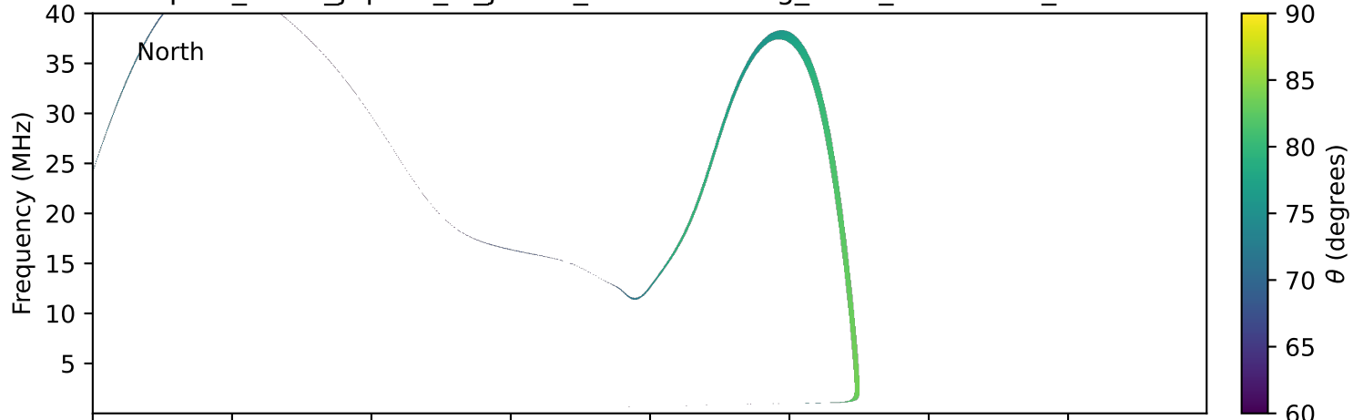
expres_earth_jupiter_io_jrm09_lossc-wid1deg_3kev_19911027_v11.cdf
