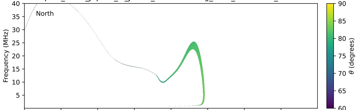
expres_earth_jupiter_io_jrm09_lossc-wid1deg_3kev_19911020_v11.cdf
