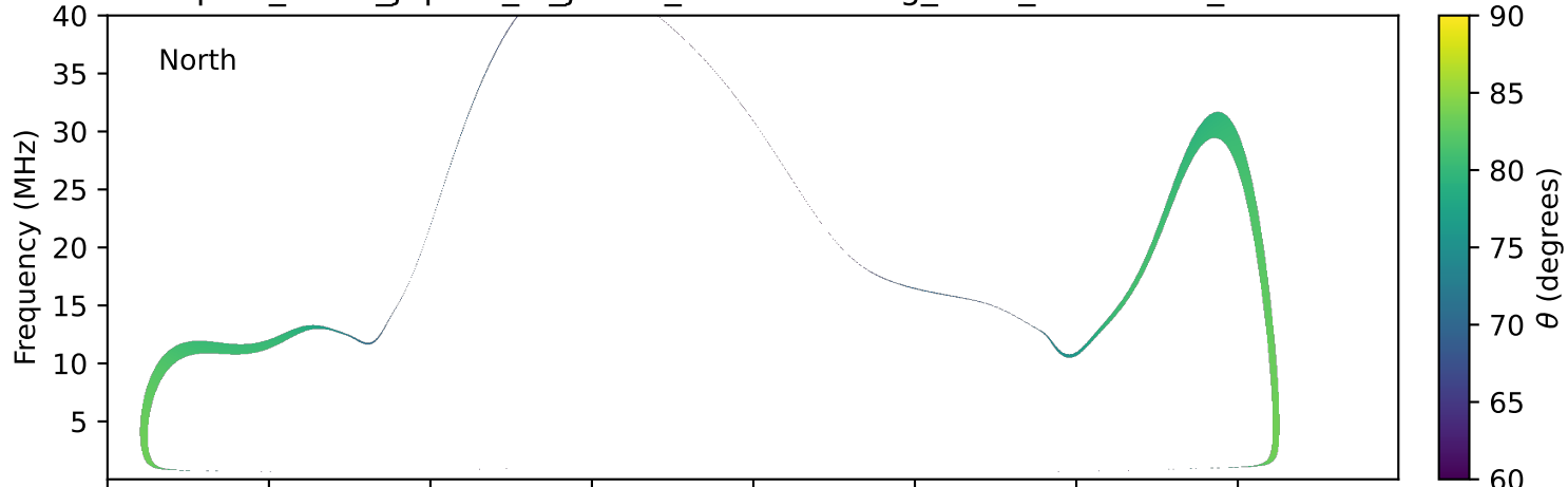
expres_earth_jupiter_io_jrm09_lossc-wid1deg_3kev_19911016_v11.cdf
