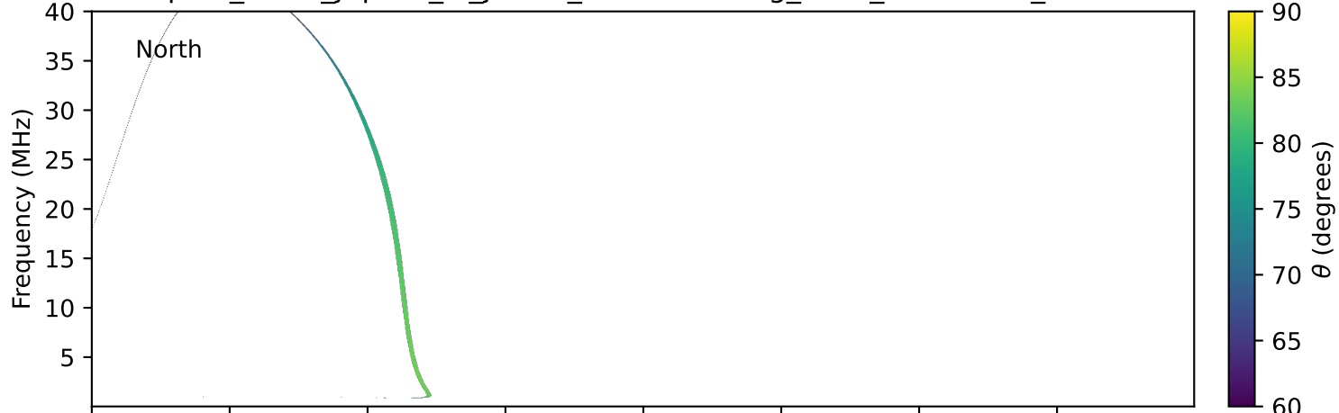
expres_earth_jupiter_io_jrm09_lossc-wid1deg_3kev_19911013_v11.cdf
