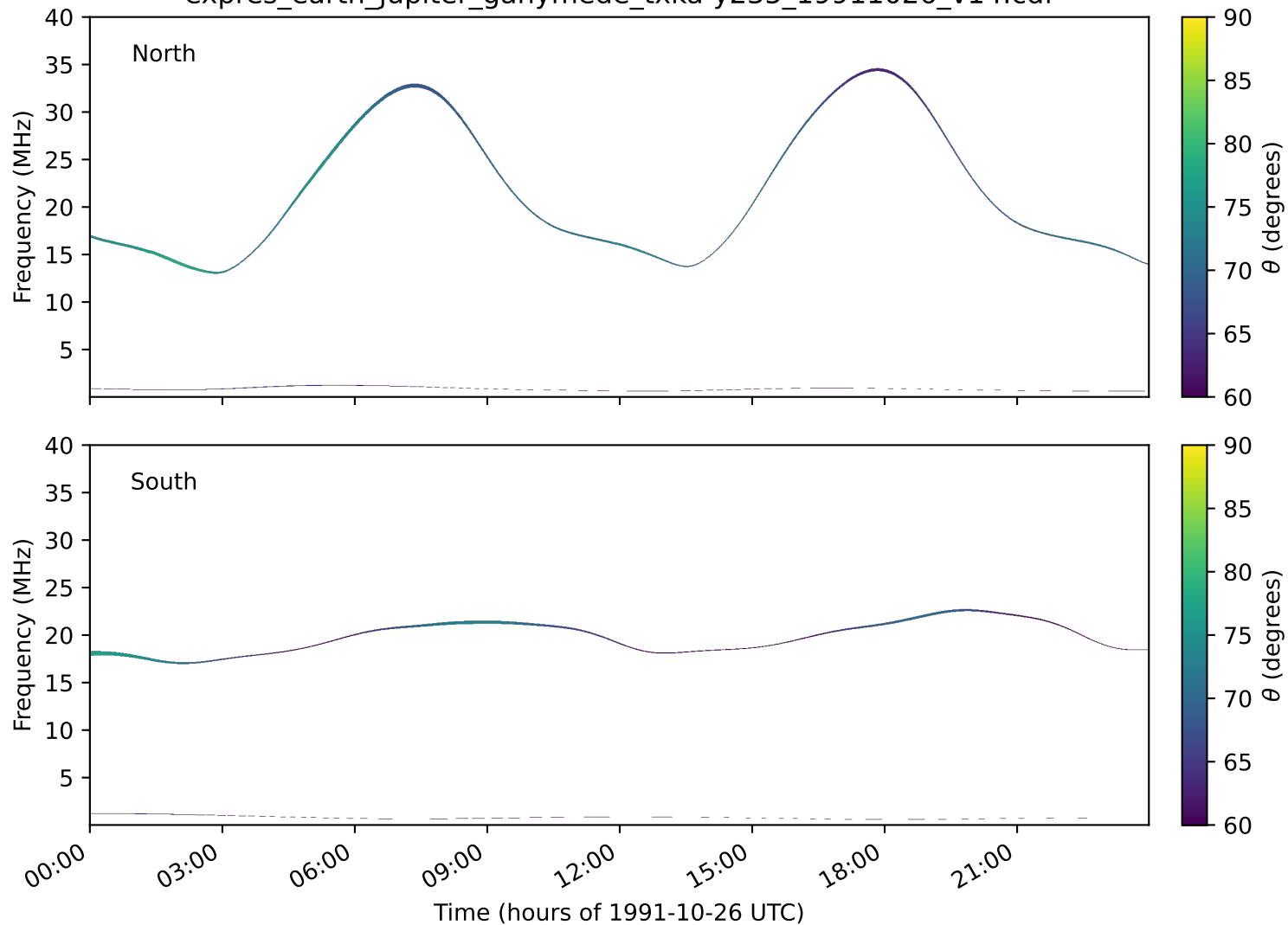
expres_earth_jupiter_ganymede_txka-y235_19911026_v14.cdf
