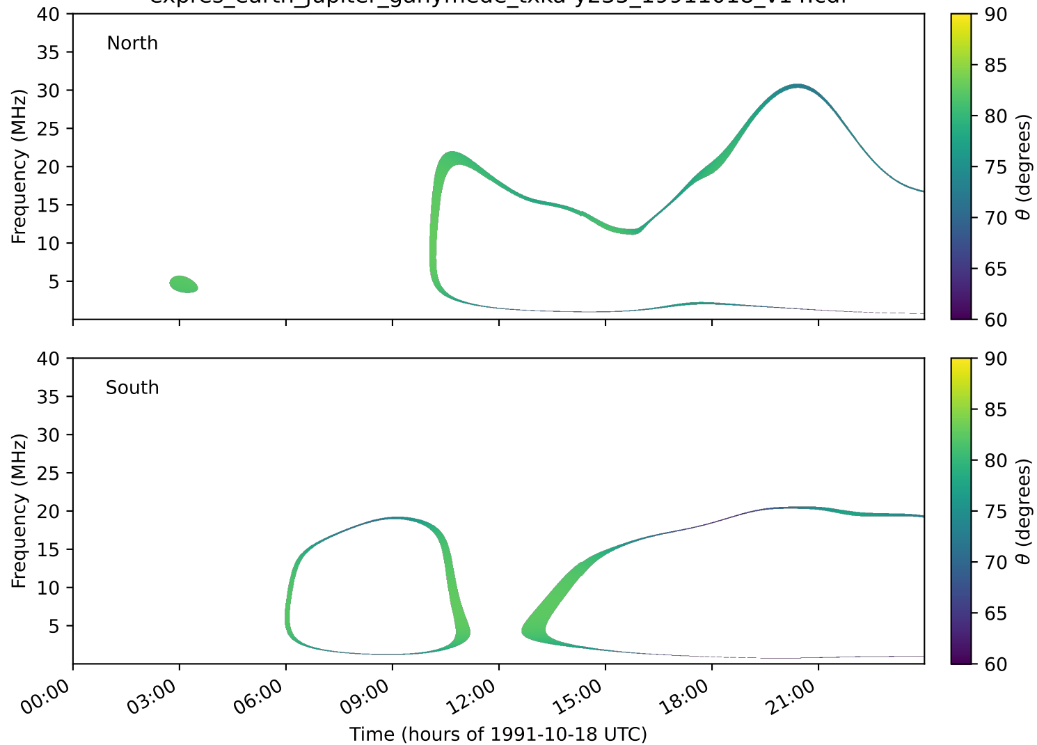
expres_earth_jupiter_ganymede_txka-y235_19911018_v14.cdf
