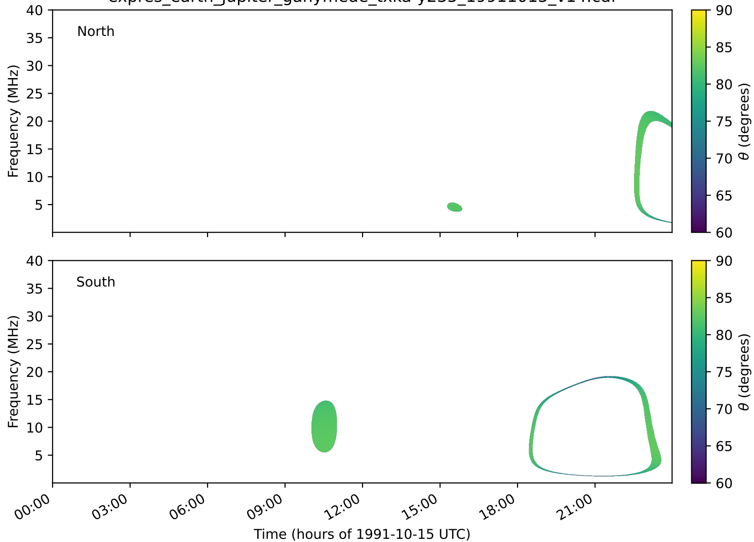
expres_earth_jupiter_ganymede_txka-y235_19911015_v14.cdf
