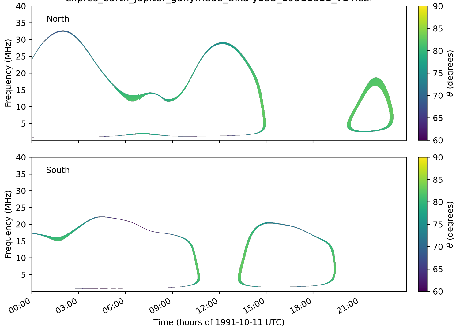
expres_earth_jupiter_ganymede_txka-y235_19911011_v14.cdf
