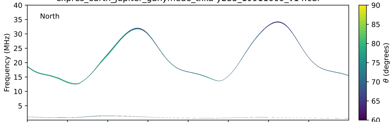
expres_earth_jupiter_ganymede_txka-y235_19911009_v14.cdf
