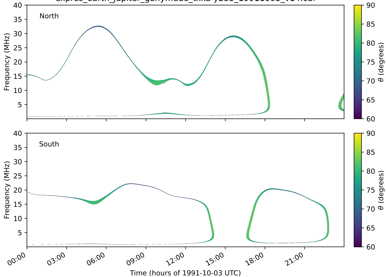
expres_earth_jupiter_ganymede_txka-y235_19911003_v14.cdf
