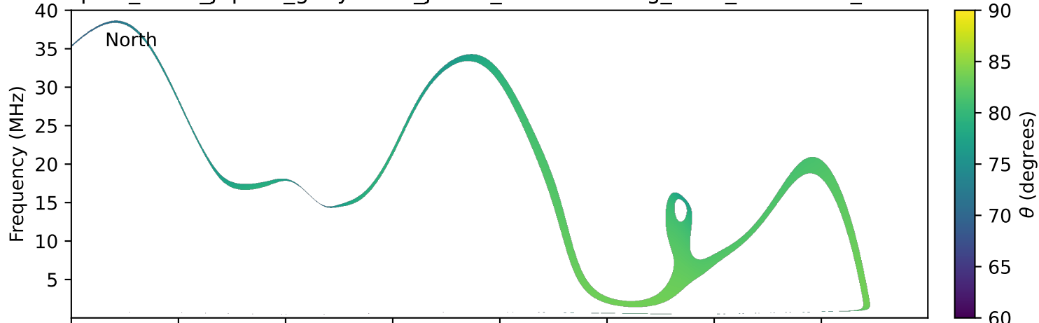
expres_earth_jupiter_ganymede_jrm33_lossc-wid1deg_3kev_19911028_v11.cdf
