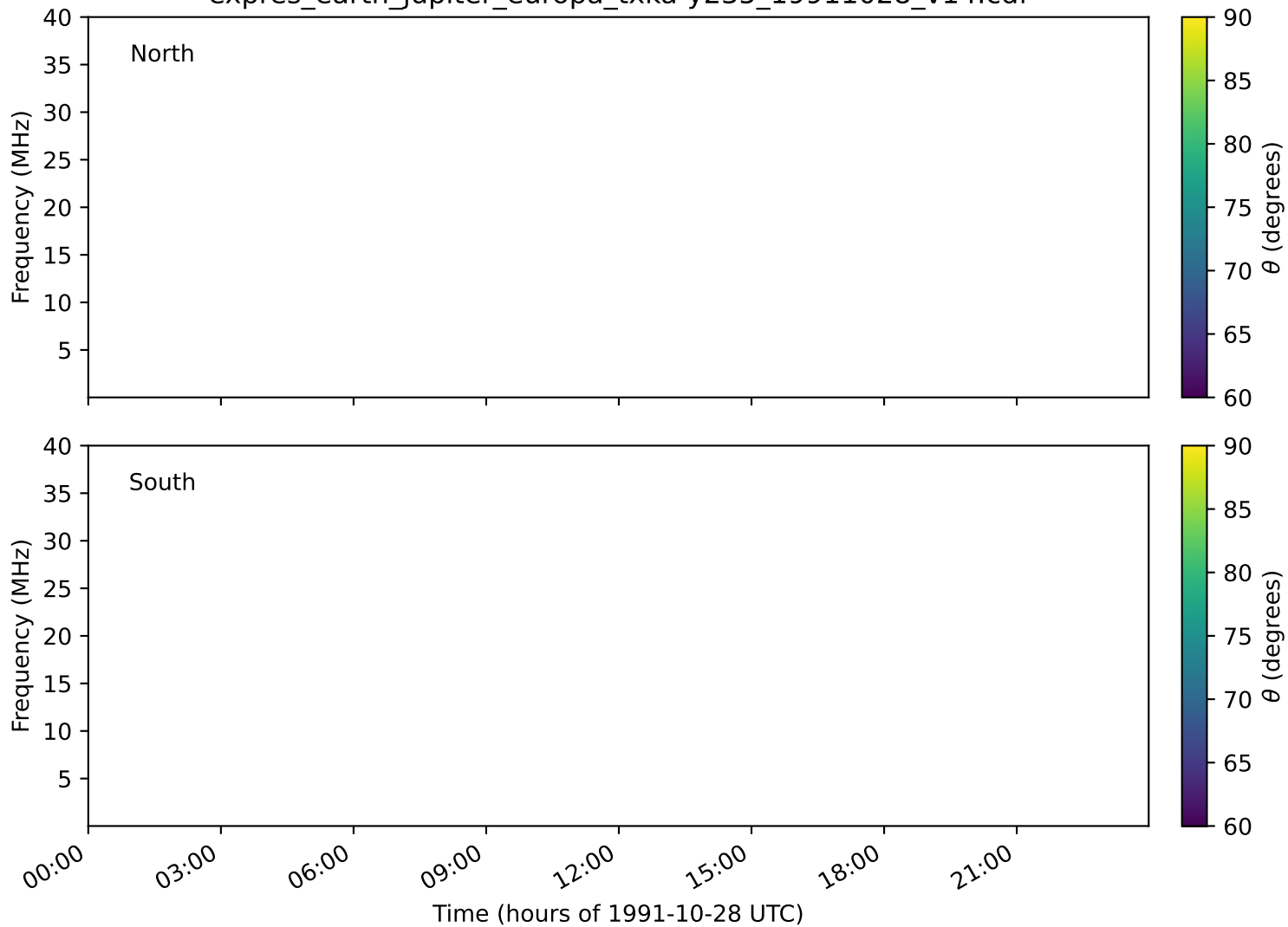
expres_earth_jupiter_europa_txka-y235_19911028_v14.cdf
