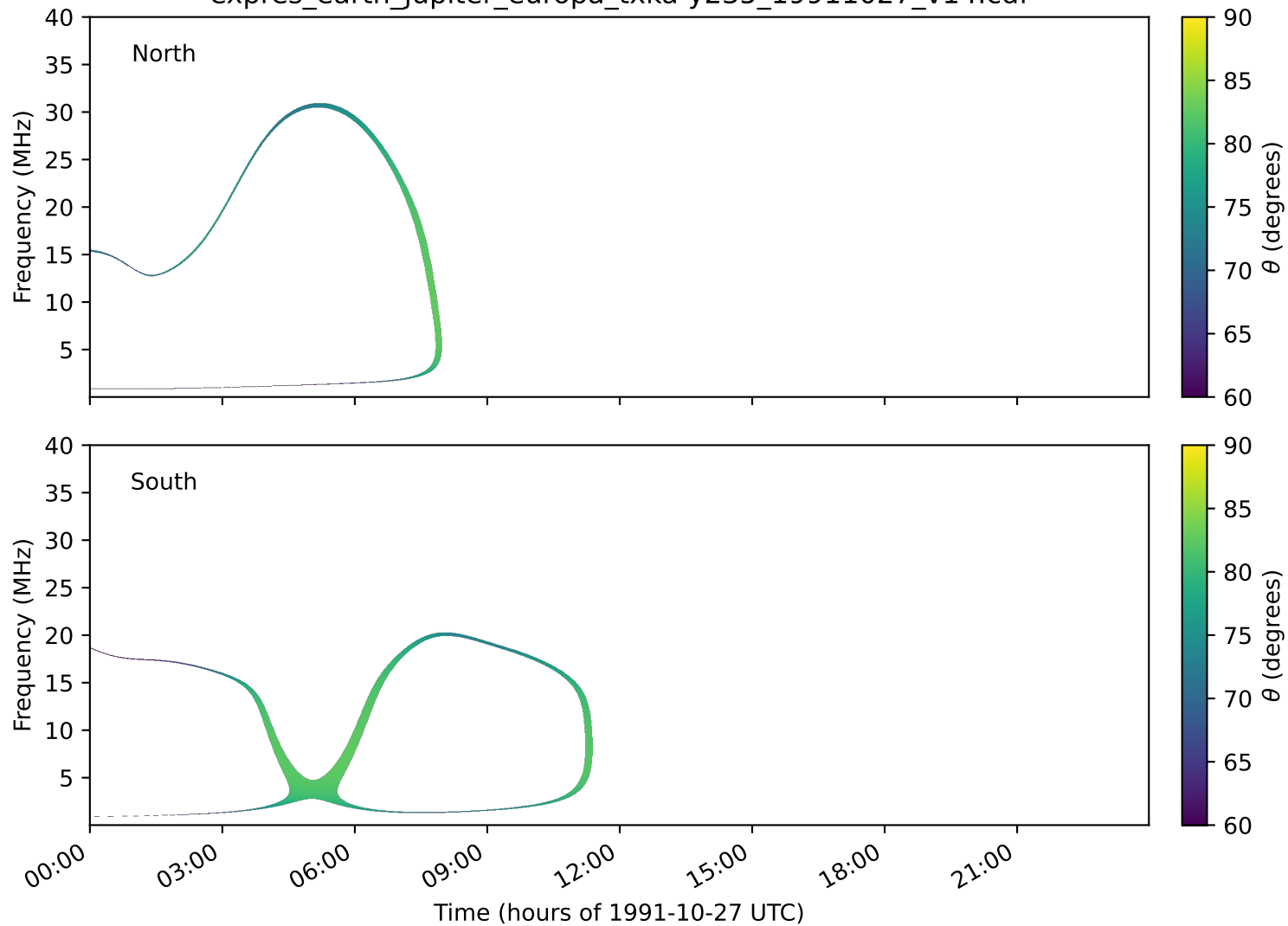
expres_earth_jupiter_europa_txka-y235_19911027_v14.cdf
