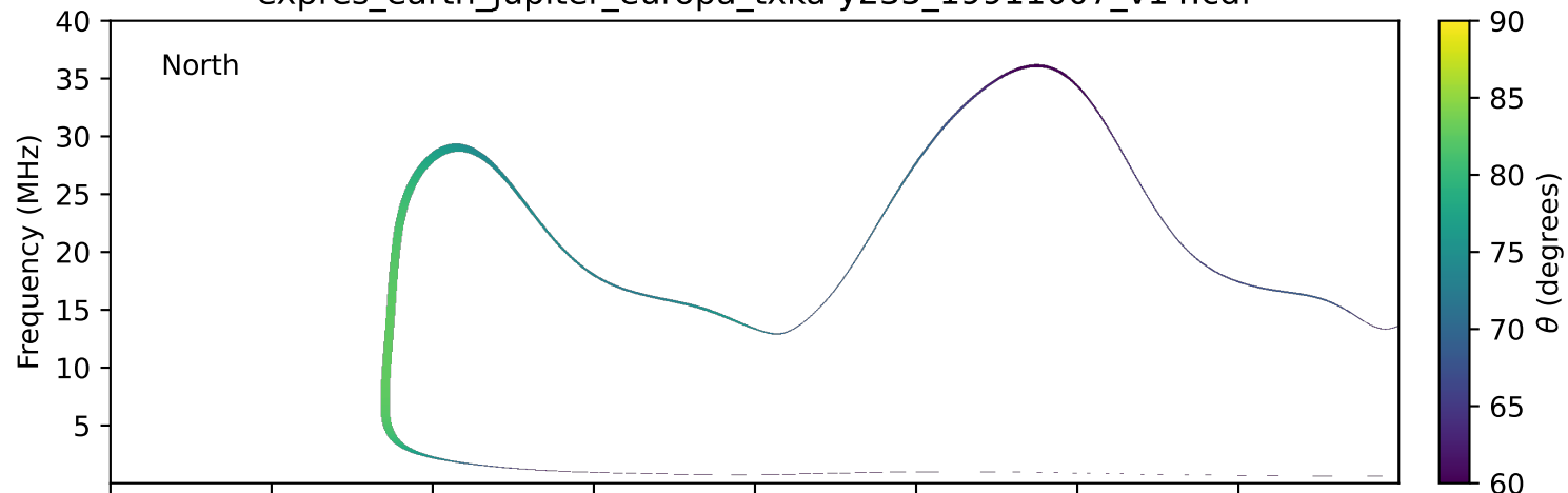
expres_earth_jupiter_europa_txka-y235_19911007_v14.cdf
