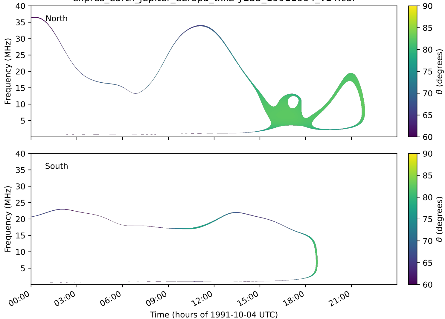
expres_earth_jupiter_europa_txka-y235_19911004_v14.cdf
