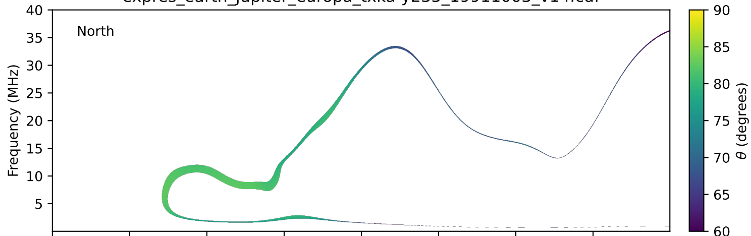
expres_earth_jupiter_europa_txka-y235_19911003_v14.cdf
