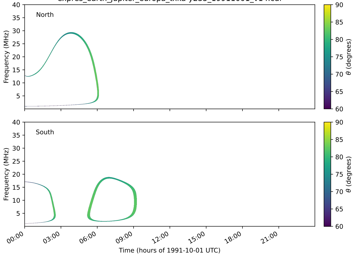
expres_earth_jupiter_europa_txka-y235_19911001_v14.cdf
