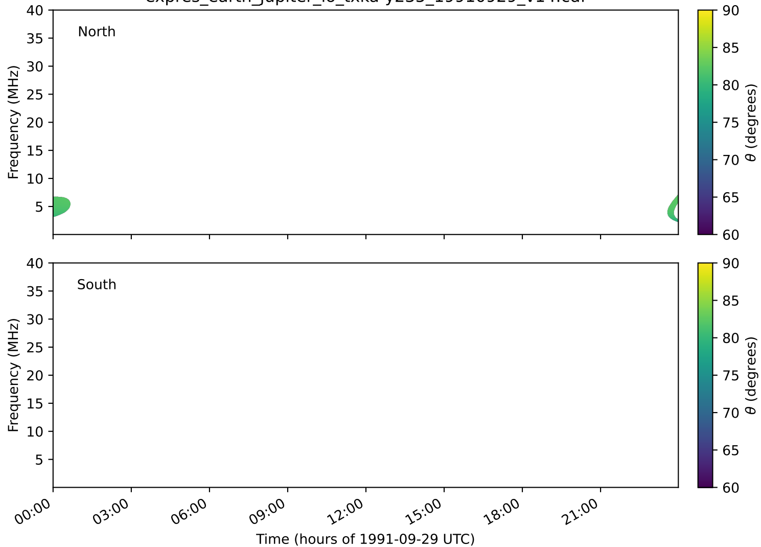
expres_earth_jupiter_io_txka-y235_19910929_v14.cdf
