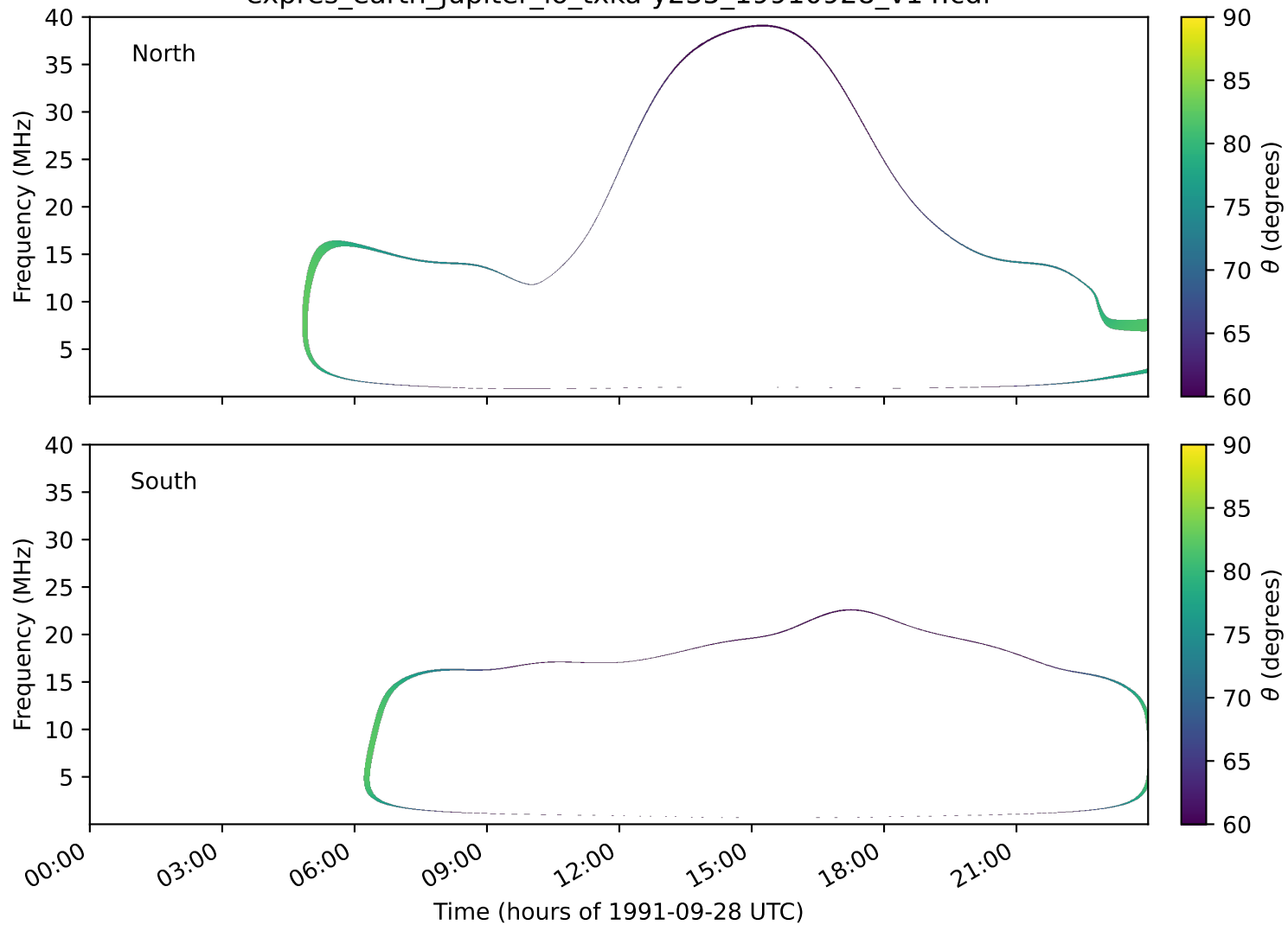
expres_earth_jupiter_io_txka-y235_19910928_v14.cdf
