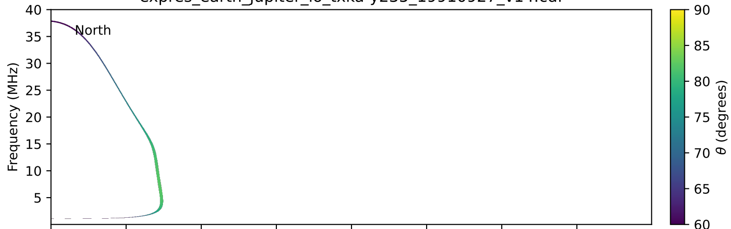
expres_earth_jupiter_io_txka-y235_19910927_v14.cdf
