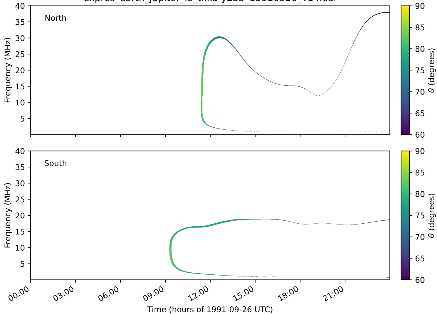
expres_earth_jupiter_io_txka-y235_19910926_v14.cdf
