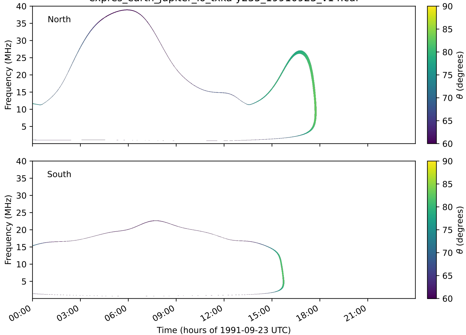
expres_earth_jupiter_io_txka-y235_19910923_v14.cdf
