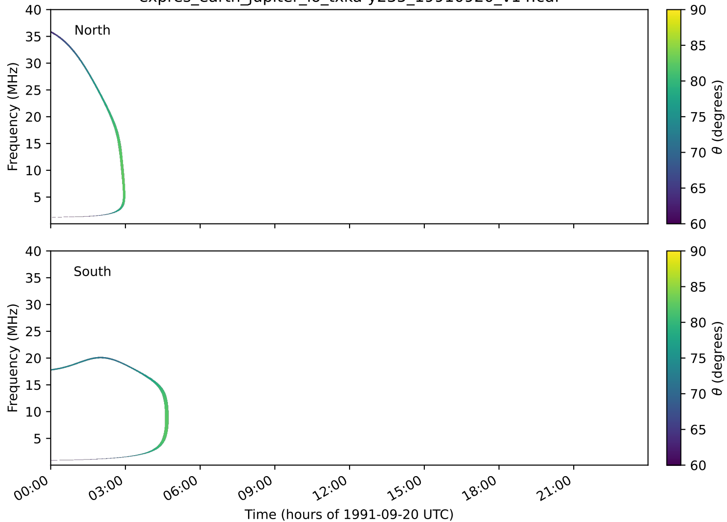
expres_earth_jupiter_io_txka-y235_19910920_v14.cdf
