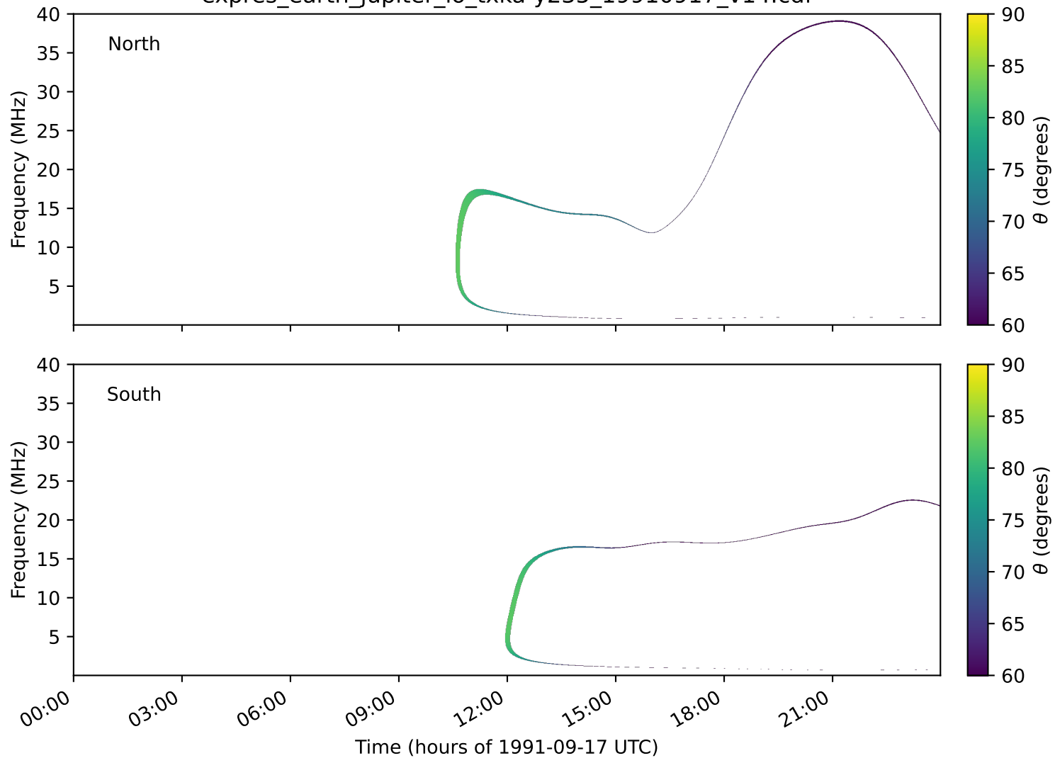
expres_earth_jupiter_io_txka-y235_19910917_v14.cdf
