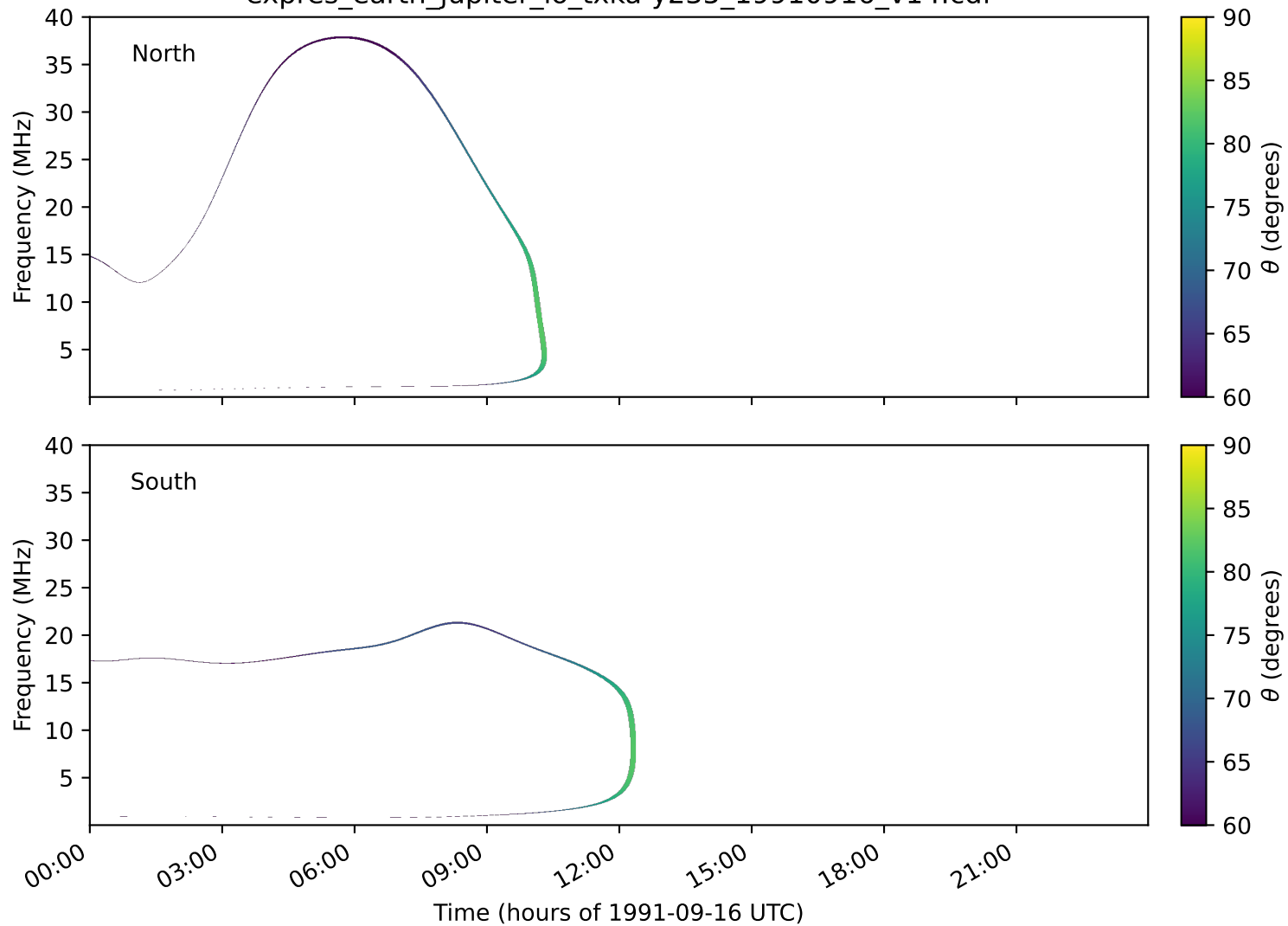
expres_earth_jupiter_io_txka-y235_19910916_v14.cdf
