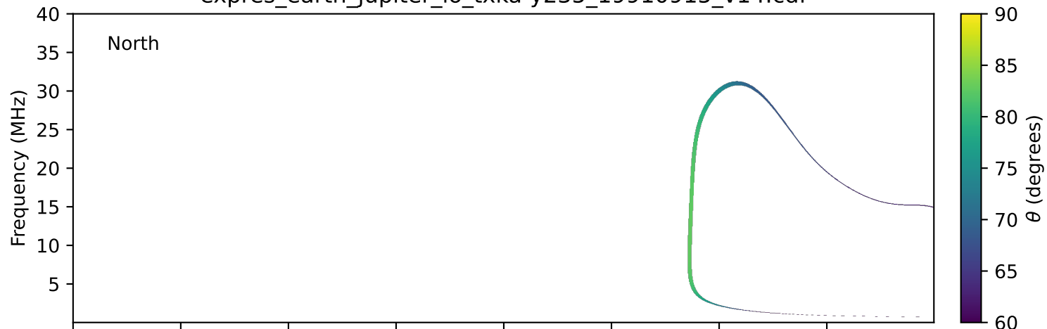
expres_earth_jupiter_io_txka-y235_19910915_v14.cdf
