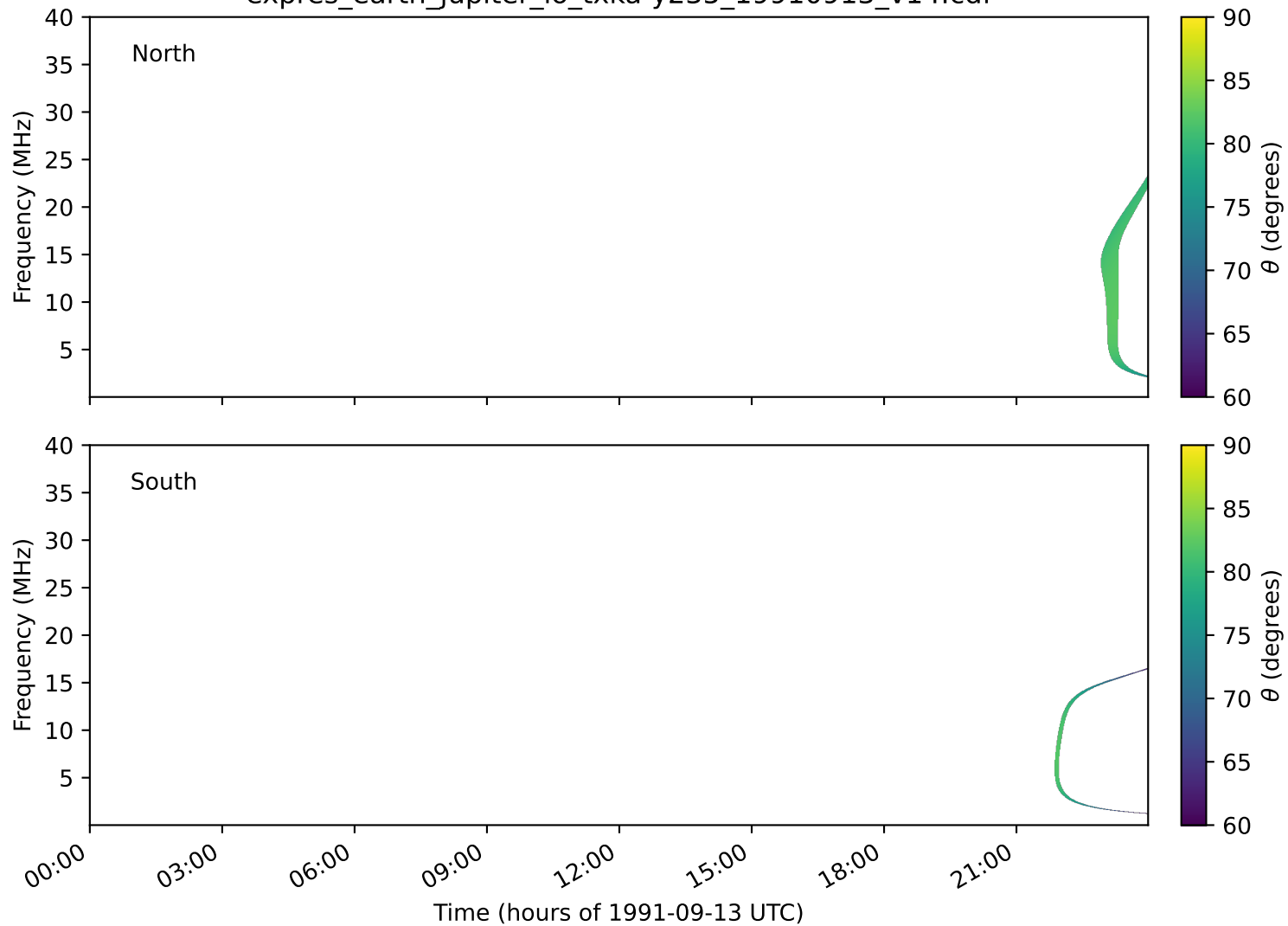
expres_earth_jupiter_io_txka-y235_19910913_v14.cdf
